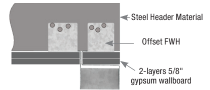
Typical FWH top flange offset, left shown (Top View)
