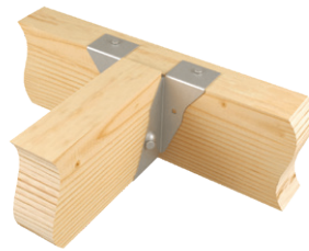
Typical JPF24 installation
