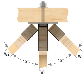
GTD top view
