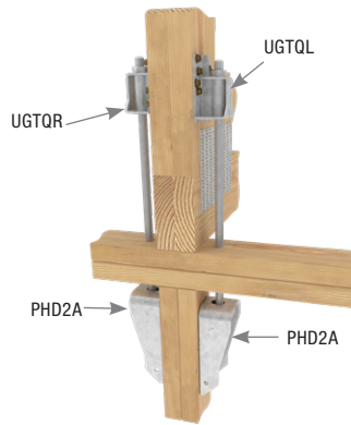
Typical UGTQL/R back-to-back installation with PHD2A
