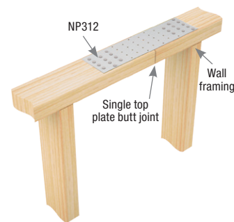
Typical NP312 prescriptive top plate splice installation
