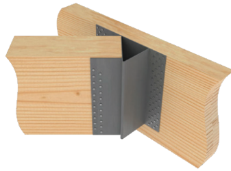
Typical THDH614-SK45RSQ installation
