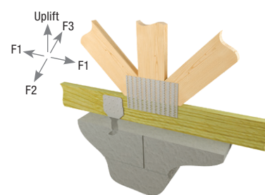
Typical LPTA parallel installation
