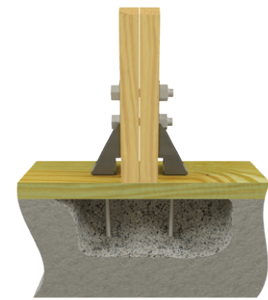
Typical TDX2-TZ back-to-back installation
