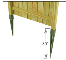
Typical SFP30 installation
