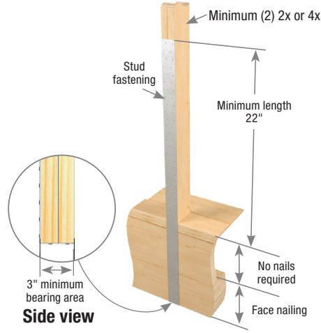
Typical MSTC66B3 installation
