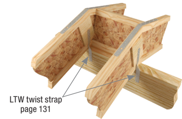
Typical LSTA/MSTA I-Joist on ridge beam installation
