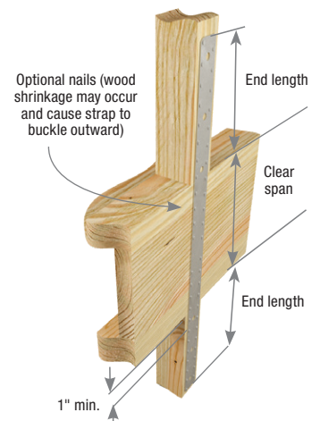
Typical KST237 floor-to-floor installation
