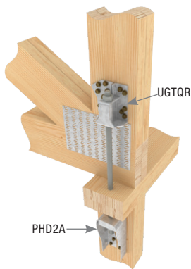
Typical UGTQ single installation with PHD2A
