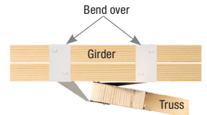
Top view right shown
