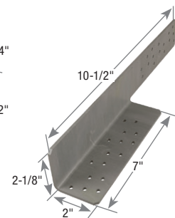
LDSC4L left shown
