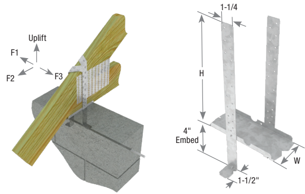
Typical DHTA 1-Ply installation
