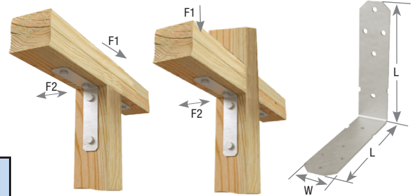
Typical B66 installations
