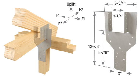
Typical LUGT2 installation
