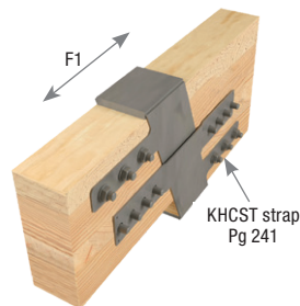
Typical KHC installation
