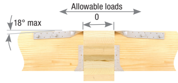
Typical KSA installation
