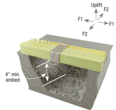
Typical FA3 standard installation in concrete
