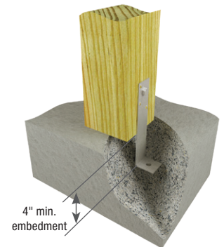
Typical TDL10 embedded bolt installation
