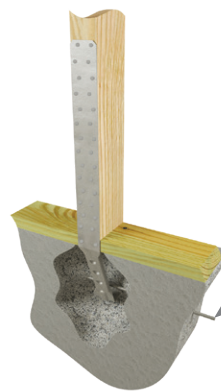
Typical STAD10 midwall installation
