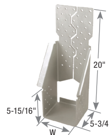
GTQ420 (GTQM420 similar)
