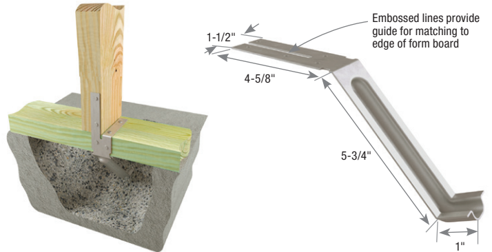
Typical FA3 one-tab-up installation
